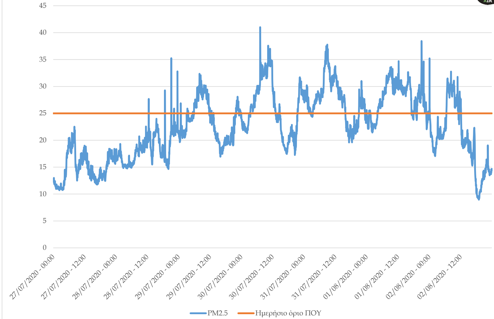
Daily mean values of PM2.5 from 27/07/2020 to 02/08/2020 in the region of Volos
