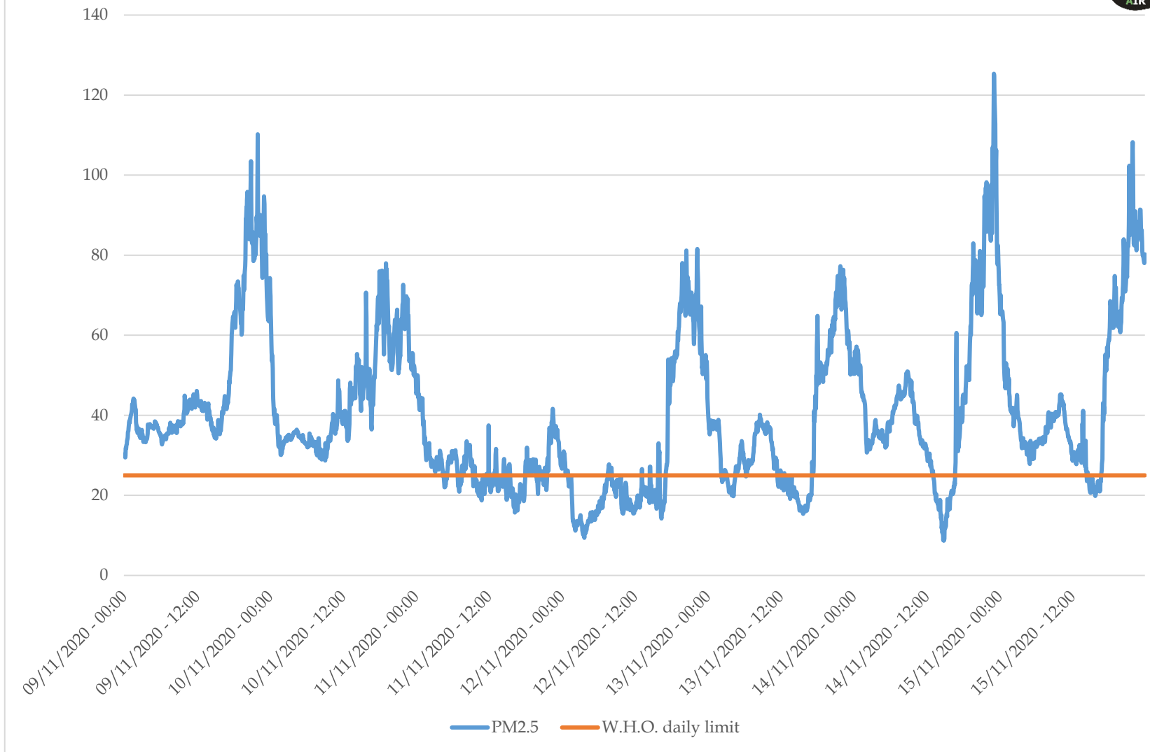
Daily mean values of PM2.5 from 09/11/2020 to 15/11/2020 in the region of Volos
